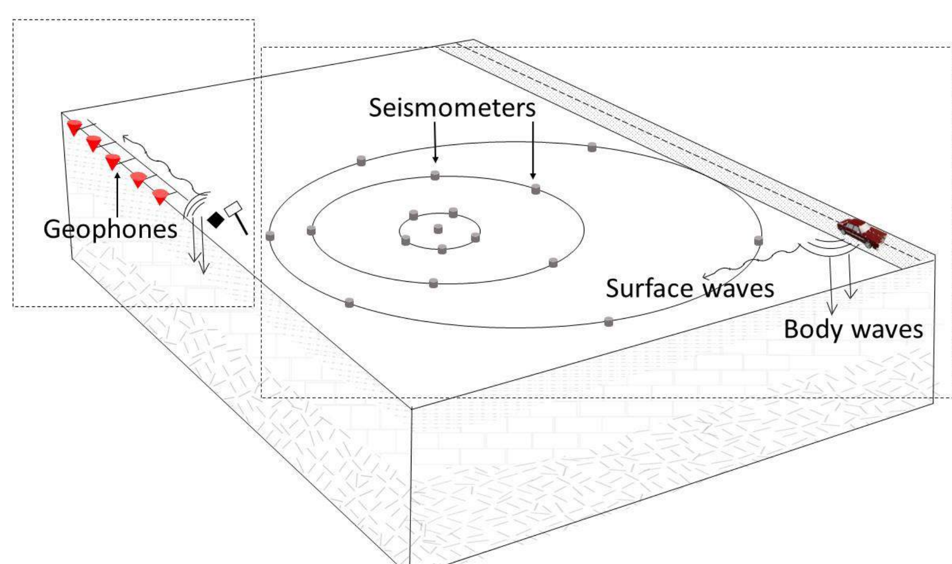
Figure 3. A schematic of the field testing setup for Microtremor Array Measurement (MAM) and Multichannel Analysis of Surface Waves (MASW). The geometry and number of arrays can vary depending on the site.
