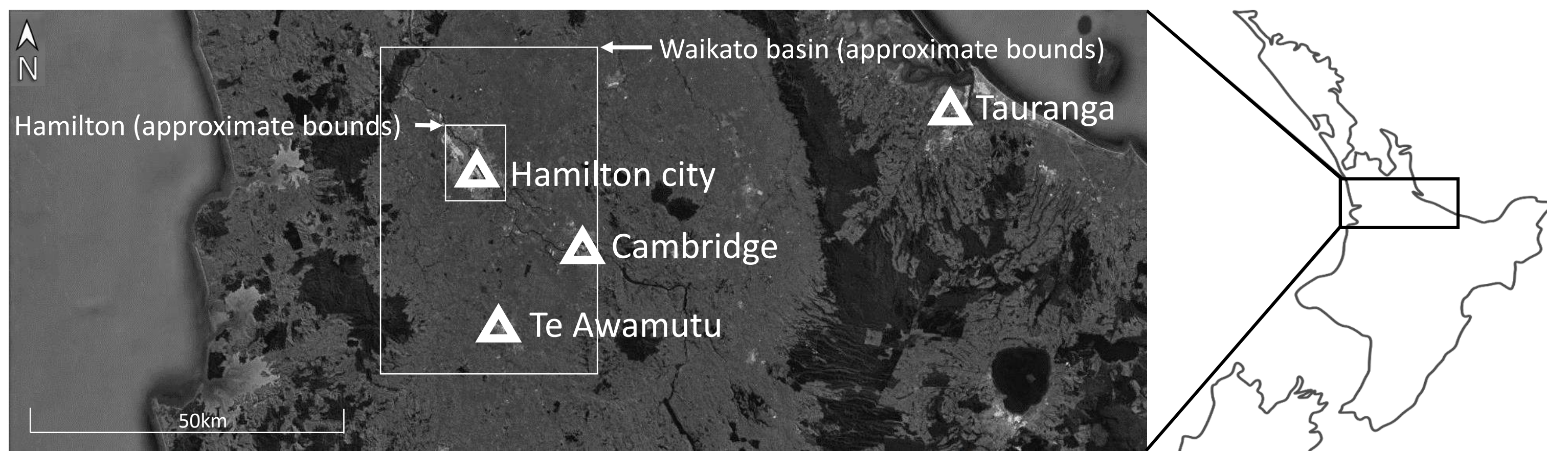
Figure 1. Location of the Waikato basin is defined by the larger rectangle with Hamilton city bounds defined by the smaller rectangle. Place names and a graphic of the North Island are included for clarity
